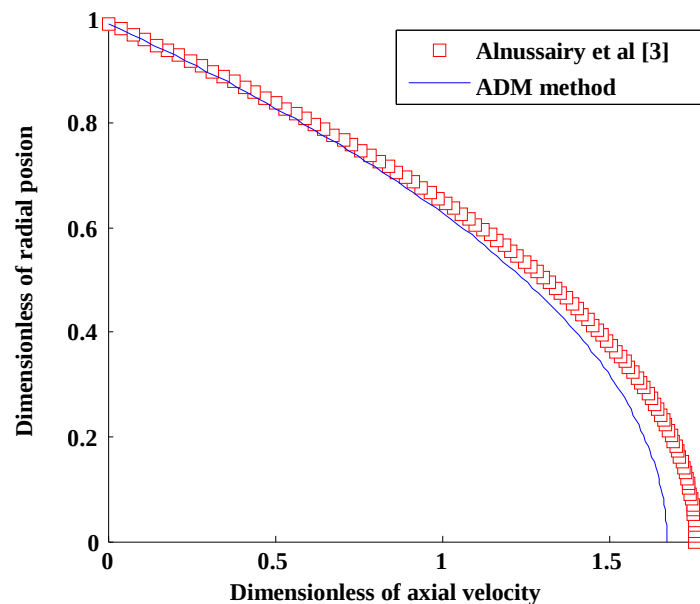
Figure 2. Comparison of axial velocity profiles in the horizontal straight trachea with Alnussairy et al. [3] at Re = 1200
