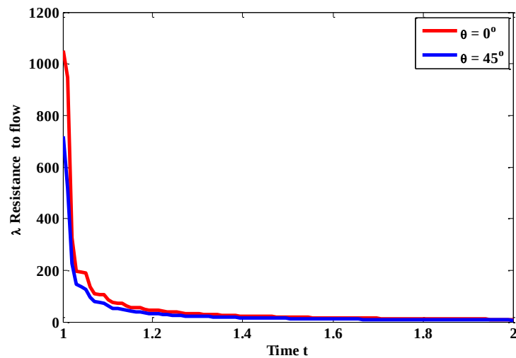
Figure 9. Variation of \lambda for a different angle at Re = 1200 and Fr=0.25 at t=1 .
