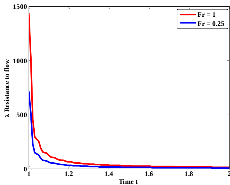
Figure 11. Variation of \lambda for a different Fr when Re = 1200 and \theta=30^\circ at t=1 .
