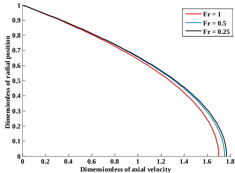
Figure 5. Axial velocity profile for different Fr at Re = 1200 and \theta = 30^\circ
