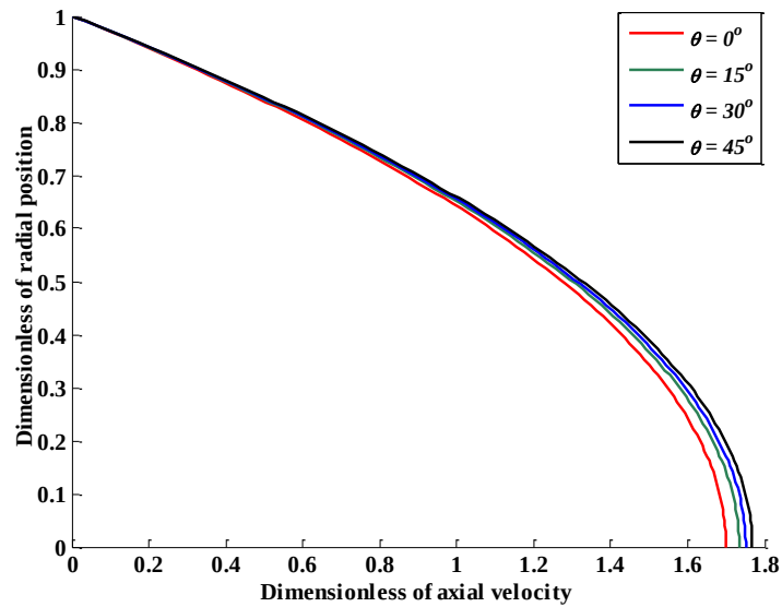
Figure 3. Variation of axial velocity profiles for different angle position at t=1 and Re = 1200 with Fr=0.27
