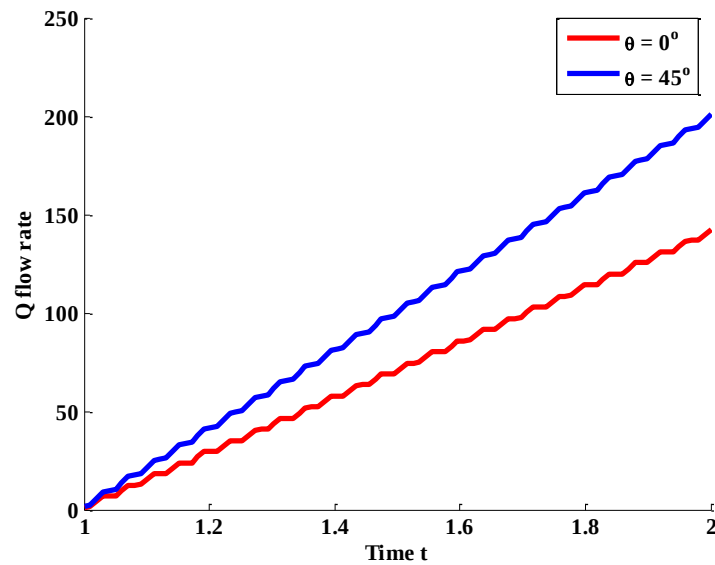
Figure 6. A variation of Q for different \theta at Re=1200 and Fr=0.25 at t=1
