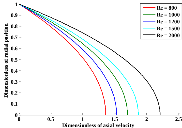
Figure 4. Variation of axial velocity profiles for different Re at t=1 and \theta = 0^\circ .
