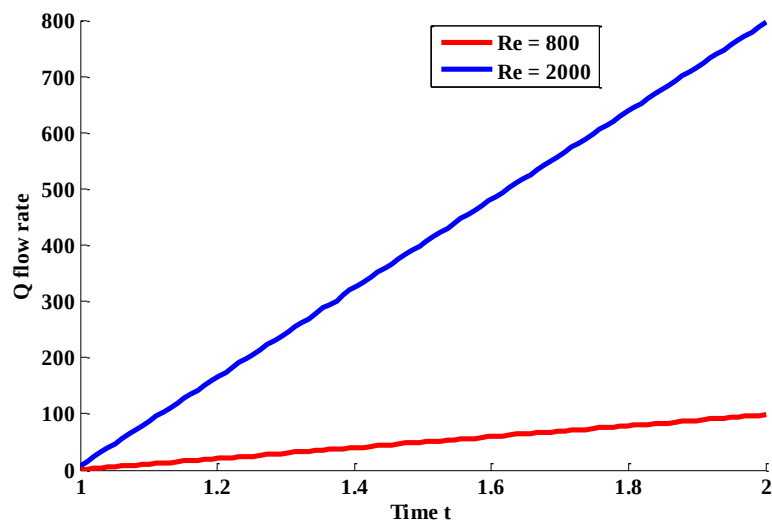
Figure 7. A variation of Q for different Re and \theta=0^\circ at t=1
