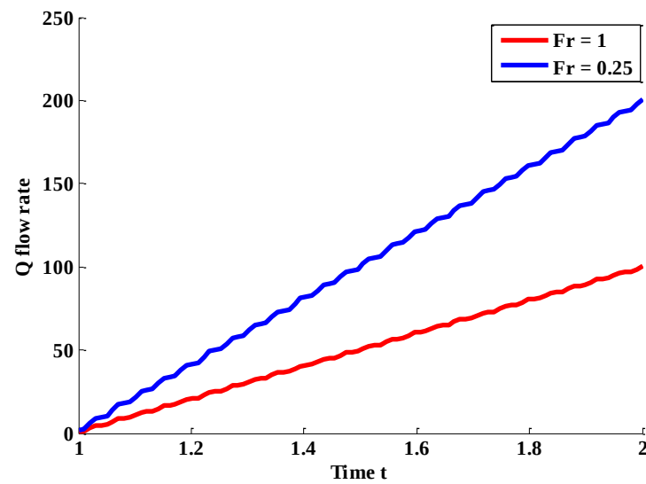
Figure 8. A variation of Q for different Fr when Re=1200 and \theta=30^\circ at t=1
